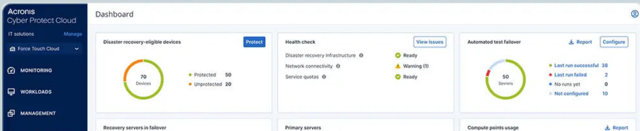
Backup and continuity readiness dashboard
